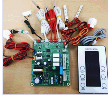
PCB AND DISPLAY
